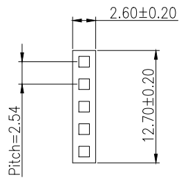
HOUSING
