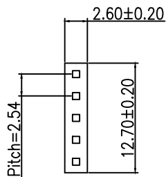
HOUSING
