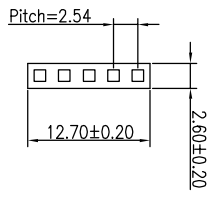
HOUSING
