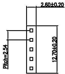
HOUSING
