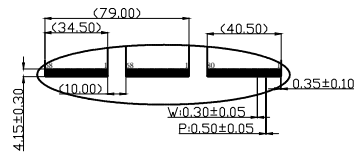
Gold finger Detail A Scale 3:1
